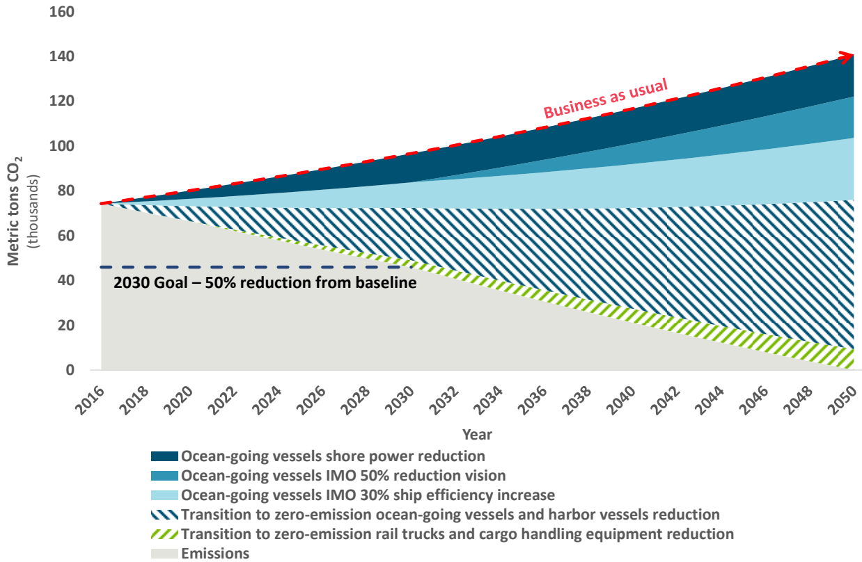
Figure ES-4. Maritime Activity future GHG emissions projection and 2050 reduction potential
